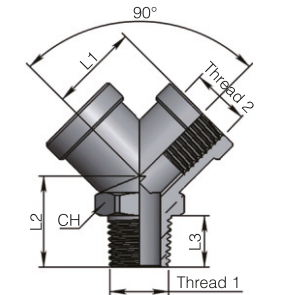
PYM Female-male Y adaptor
