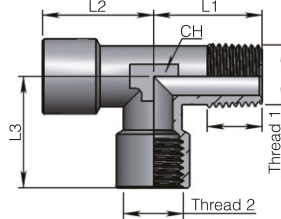
PMFS Female-female-male tee adaptor
