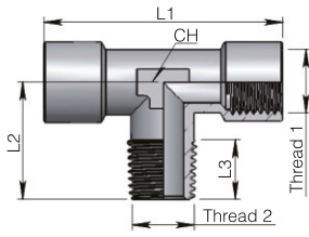
PMT Female-male-female tee adaptor
