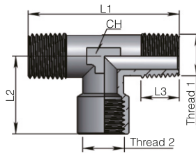
PMSM Male-female-male tee adaptor
