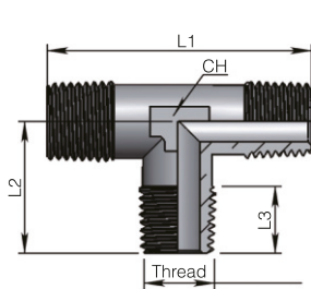
PMS Male tee adaptor
