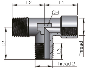
PMSF Male-male-female tee adaptor
