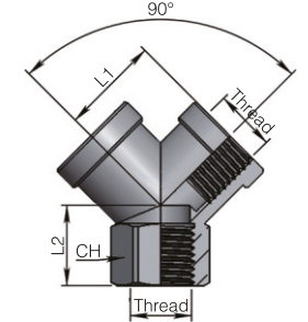
PYF Female Y adaptor
