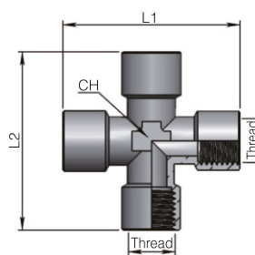
PFC Female cross adaptor
