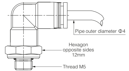
Standard type
