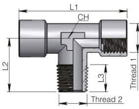
PMT Female-male-female tee adaptor
