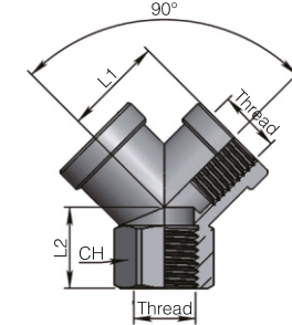
PYF Female Y adaptor
