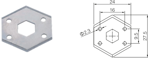
TC-B-B Tube cutter B type blade
