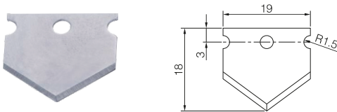
TC-A-B Tube cutter A type blade
